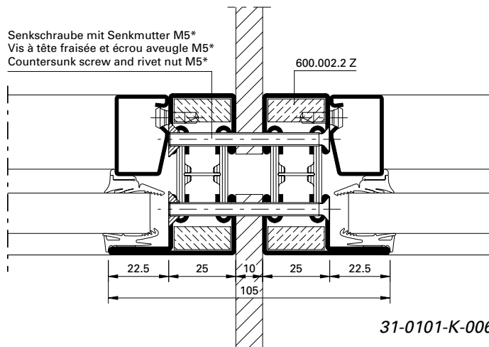
Junction detail
