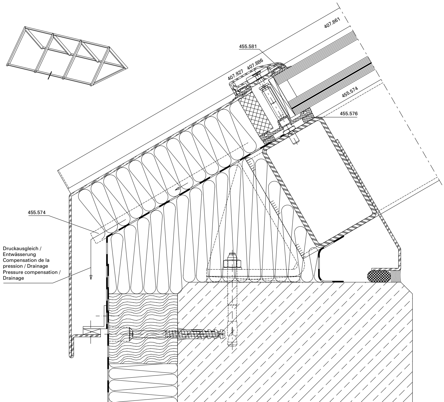
Base point attachment detail
